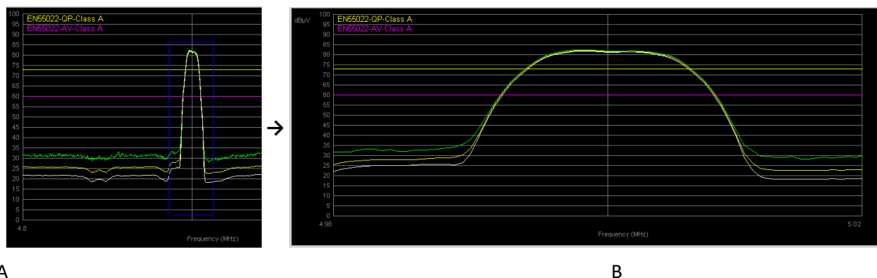
Fig. D.57: Manual Zoom on Emission Spectrum
