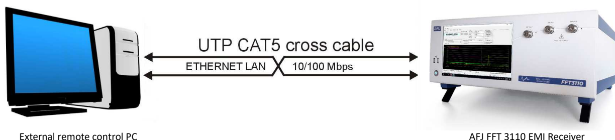
Fig. C.1: Connection procedure for FFT 3110 EMI receiver
