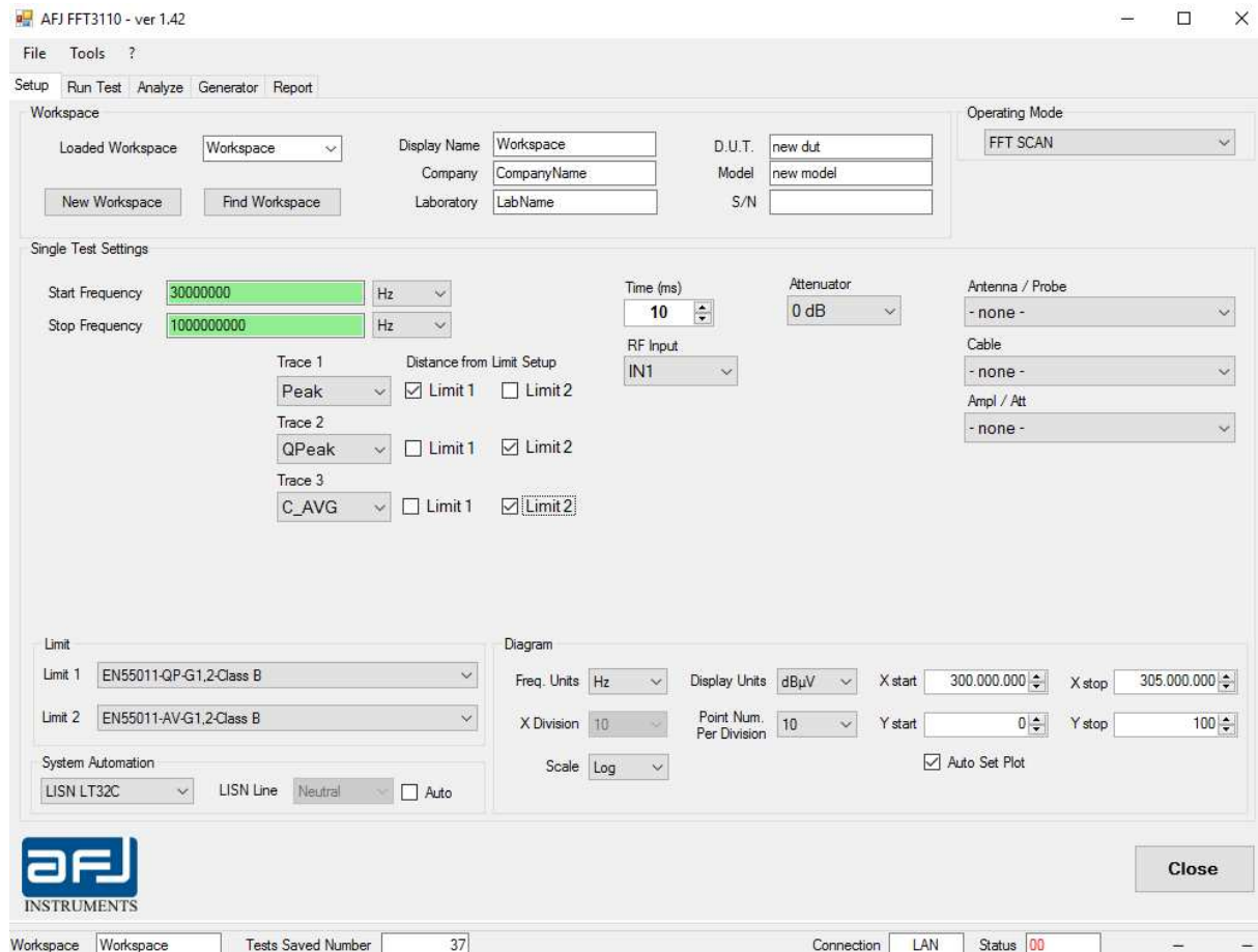
Fig. D.1: The Setup box of the FFT 3110 EMI Receiver cockpit
