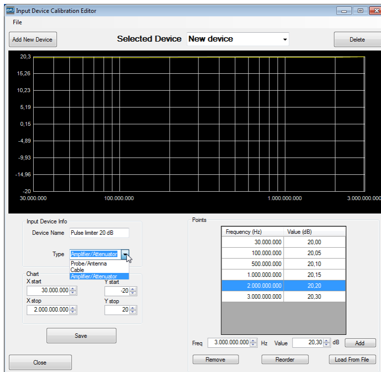
D.25: Input Device Calibration parameters for an external 20 dB Attenuator
