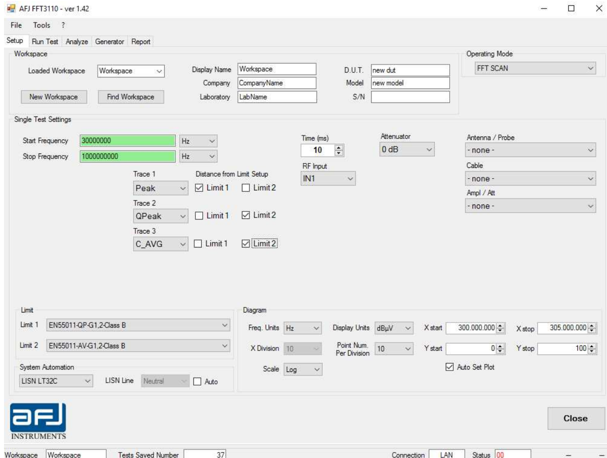
Fig. D.2: FFT 3110 EMI Receiver setup window
