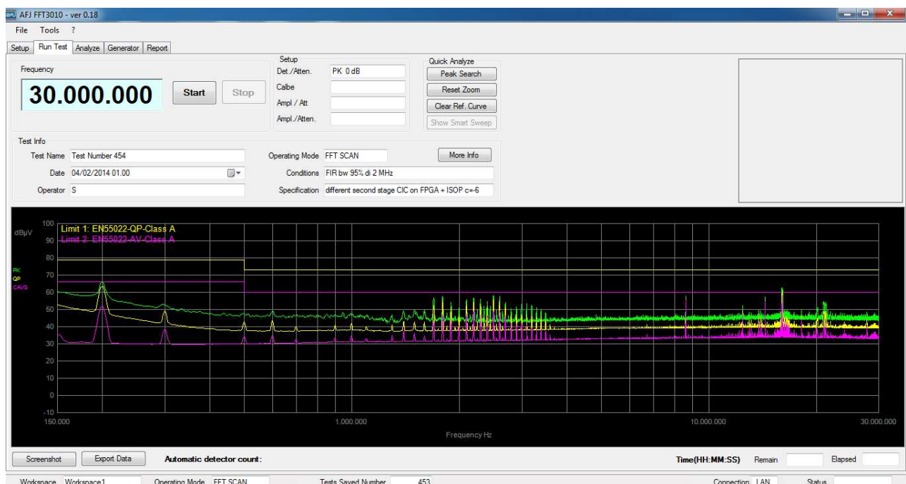
Fig. D.52: A frequency spectrum of conducted emission measurement from 150 kHz to 30 MHz
