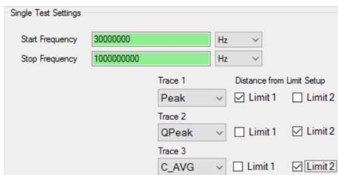
Fig. D.7: Setup of the Single Test Settings section for FFT Scan Mode with three traces at once
