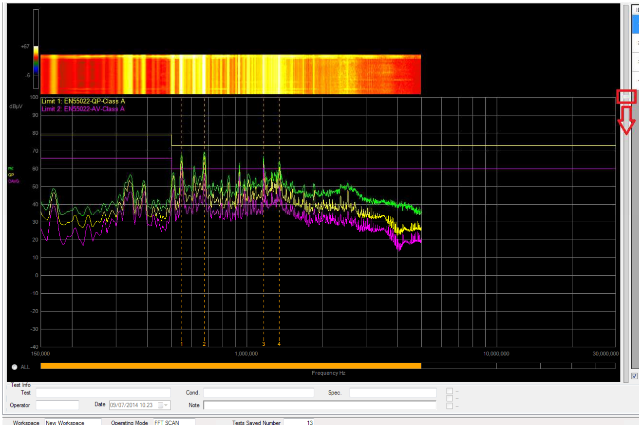
Fig. D.87: Waterfall visualization
