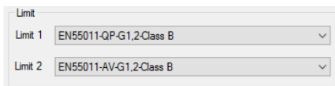
Fig. D.8: Selection of limits in the Limit section
